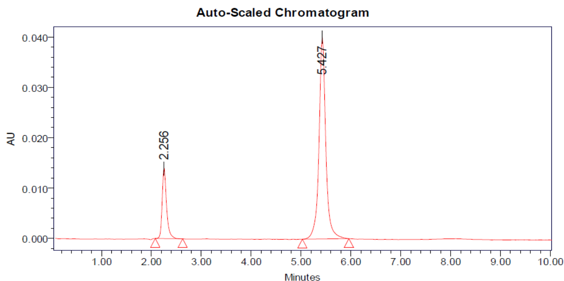
Fig 1: Optimized Chromatogram
