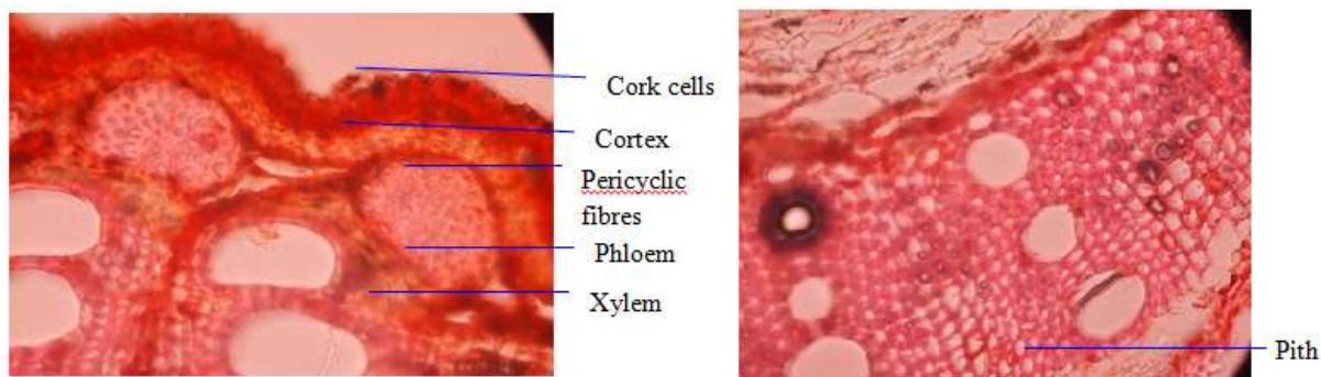
Fig 3b: Detailed TS of Ampelocissus latifolia stem
